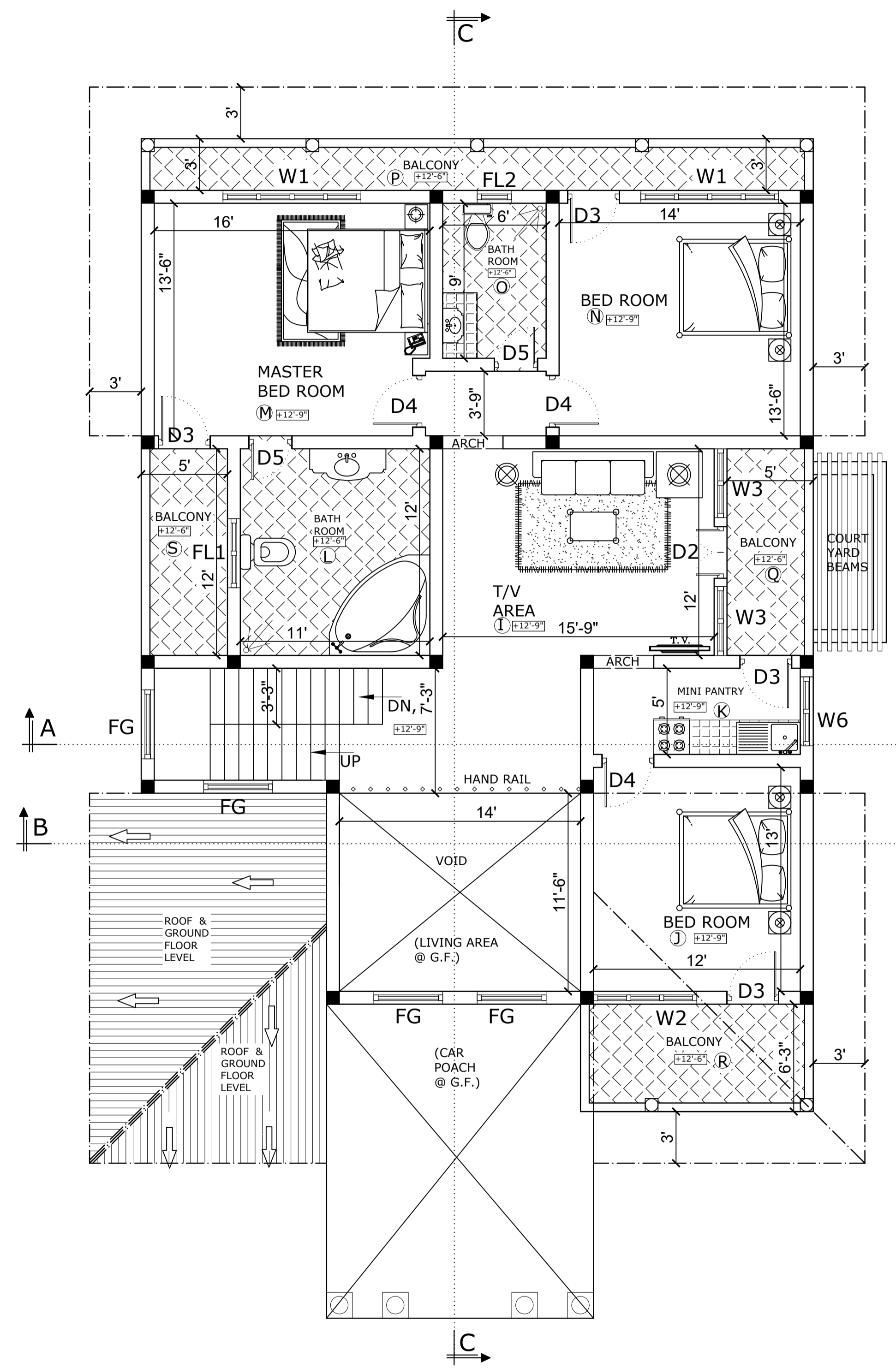
FIRST FLOOR PLAN Scale 0'-1/8" : 1'-0"
