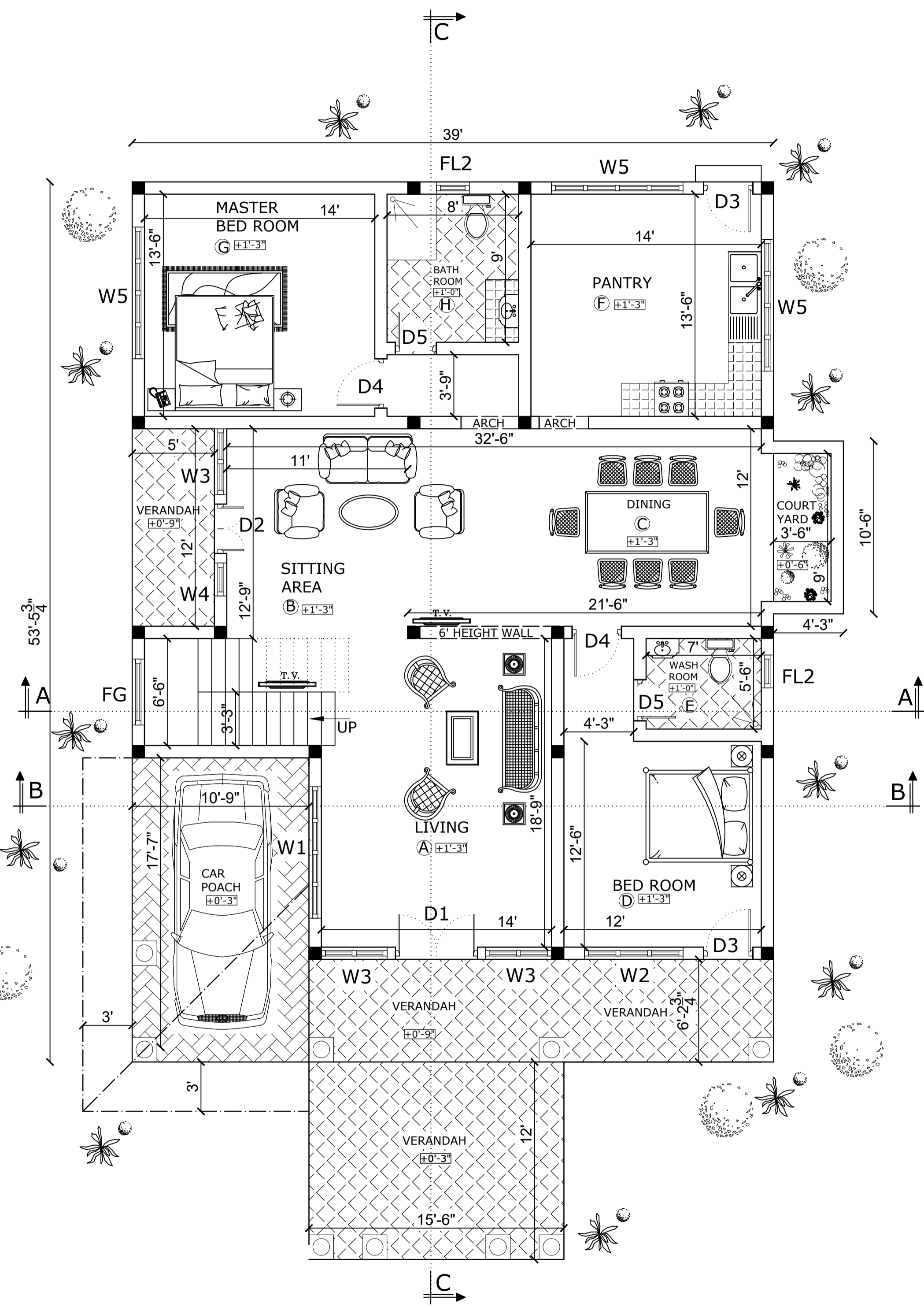
GROUND FLOOR PLAN Scale 0'-1/8" : 1'-0"
