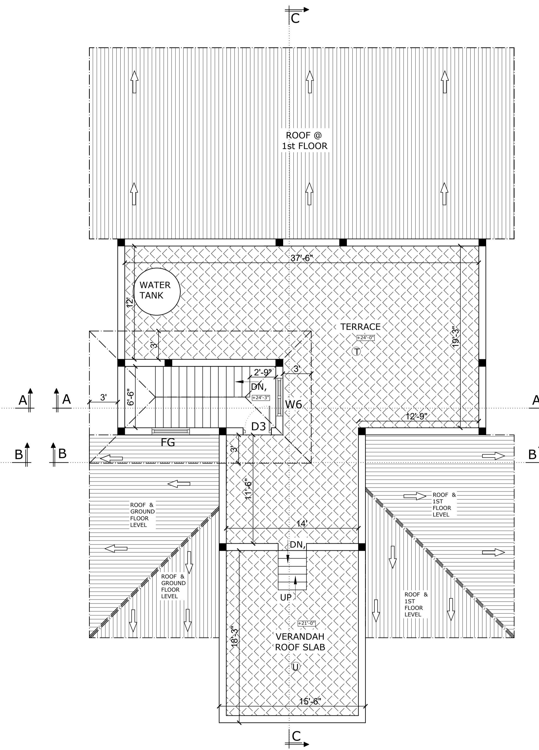
TERRACE PLAN Scale 0'-1/8" : 1'-0"
